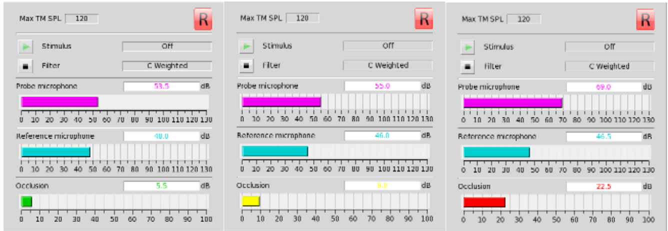
Occlusion effect measurement
