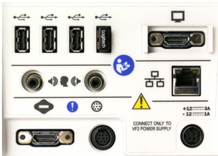
Display unit rear connector panel
